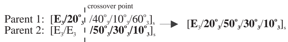
Figure 2.5: One-point crossover.
