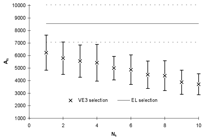
Figure 4.10: Cost comparison - EL vs. VE_3 ( P = 20 ).
