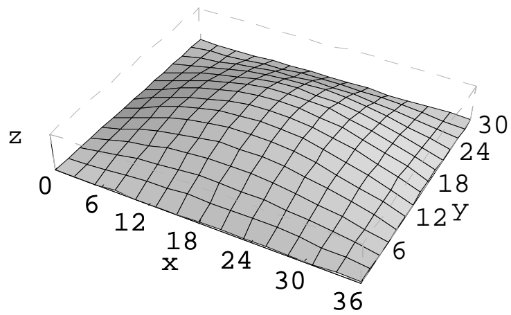
Figure 5.7: Buckling mode shapes for uniaxial loading.
